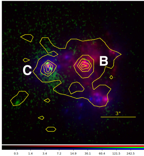
(a) Haro 11
