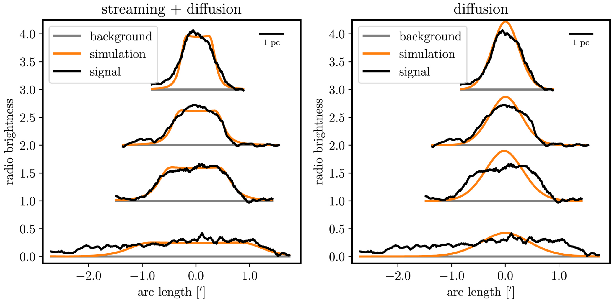
Figure 5. from Probing Cosmic-Ray Transport with Radio Synchrotron Harps in the Galactic Center null 2020 APJL 890 L18 doi:10.3847/2041-8213/ab7237 https://dx.doi.org/10.3847/2041-8213/ab7237
