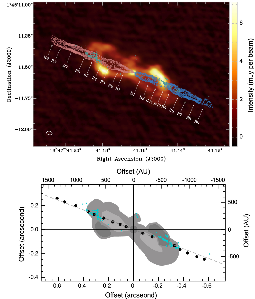
Figure 3. from Shaping the Envelope of the Asymptotic Giant Branch Star W43A with a Collimated Fast Jet null 2020 APJL 890 L14 doi:10.3847/2041-8213/ab70b8 https://dx.doi.org/10.3847/2041-8213/ab70b8 © 2020. The American Astronomical Society. All rights reserved.
