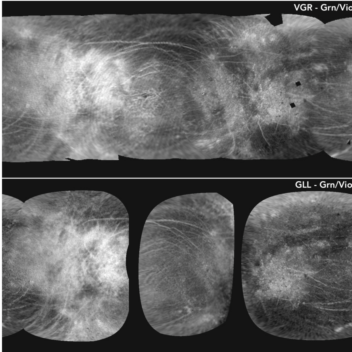
Figure 2. from The Search for Europa's Plumes: No Surface Patterns or Changes 1979–2007? null 2020 APJL 892 L12 doi:10.3847/2041-8213/ab6f78 https://dx.doi.org/10.3847/2041-8213/ab6f78 © 2020. The American Astronomical Society. All rights reserved.
