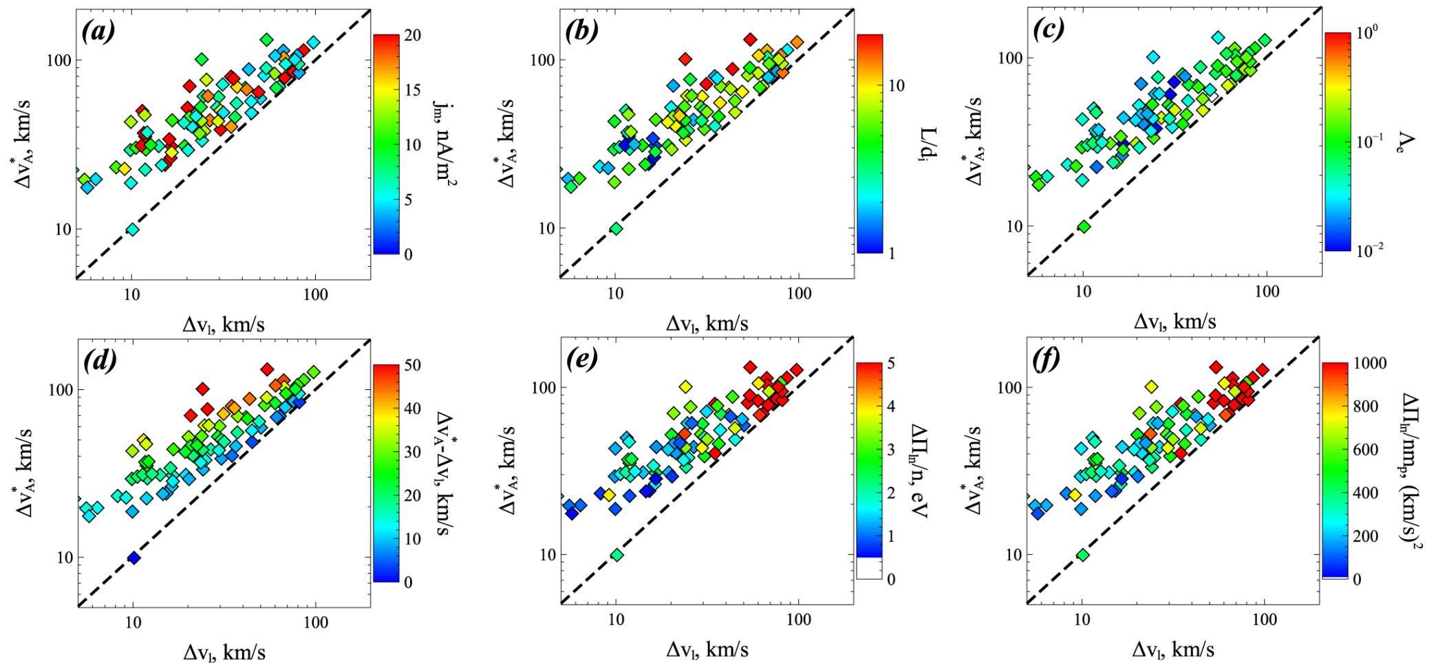
Figure 4. from Ion Nongyrotropy in Solar Wind Discontinuities null 2020 APJL 889 L23 doi:10.3847/2041-8213/ab6b2e https://dx.doi.org/10.3847/2041-8213/ab6b2e © 2020. The American Astronomical Society. All rights reserved.
