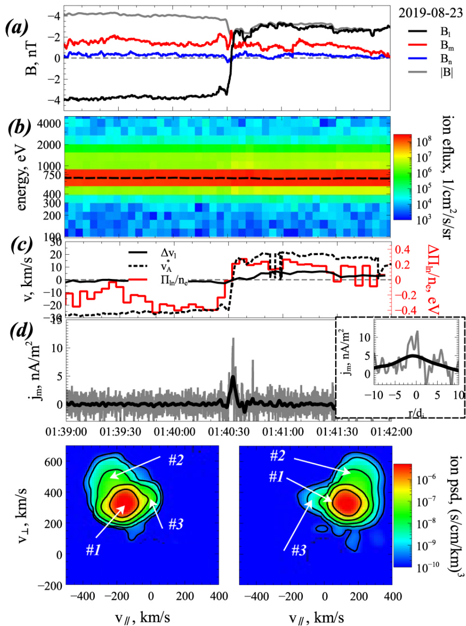
Figure 3. from Ion Nongyrotropy in Solar Wind Discontinuities null 2020 APJL 889 L23 doi:10.3847/2041-8213/ab6b2e https://dx.doi.org/10.3847/2041-8213/ab6b2e
