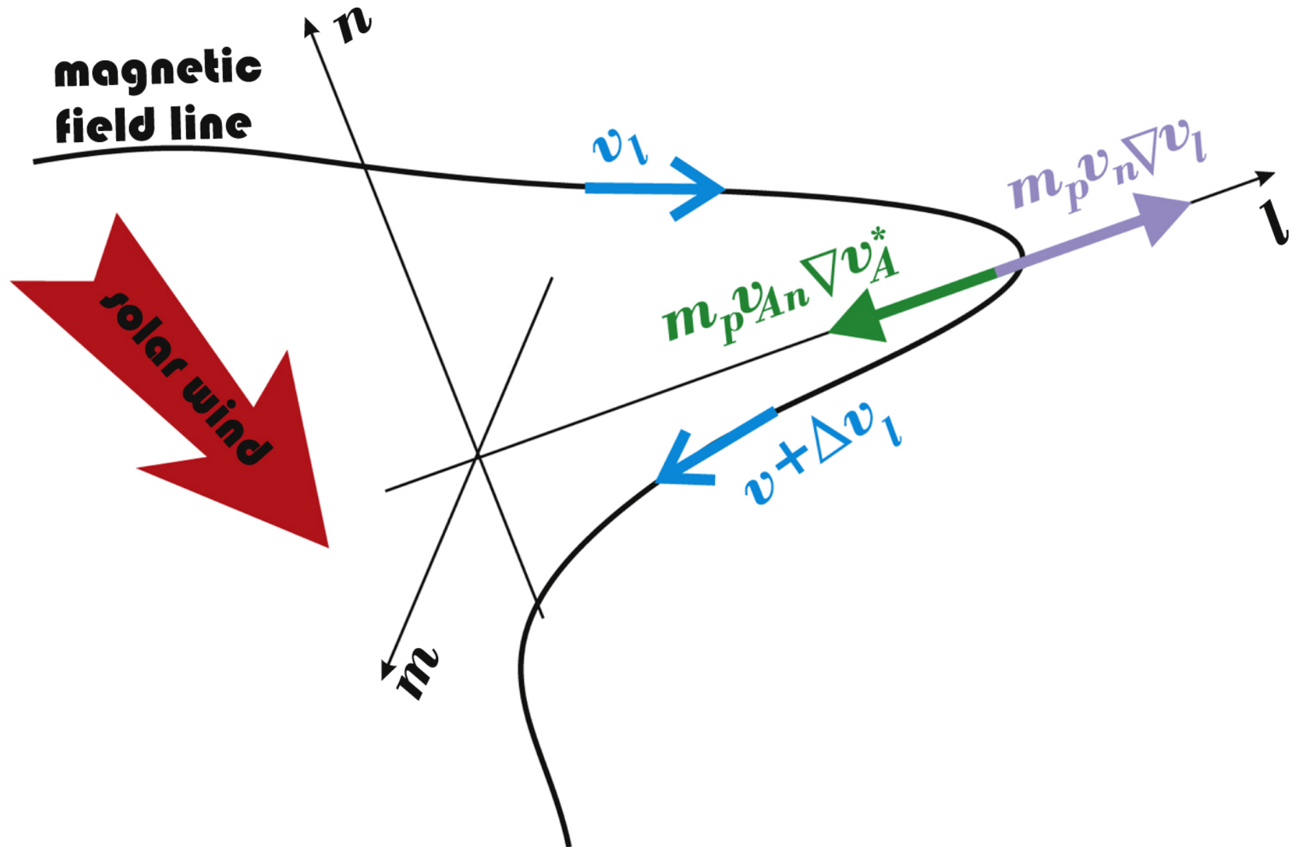
Figure 1. from Ion Nongyrotropy in Solar Wind Discontinuities null 2020 APJL 889 L23 doi:10.3847/2041-8213/ab6b2e https://dx.doi.org/10.3847/2041-8213/ab6b2e © 2020. The American Astronomical Society. All rights reserved.
