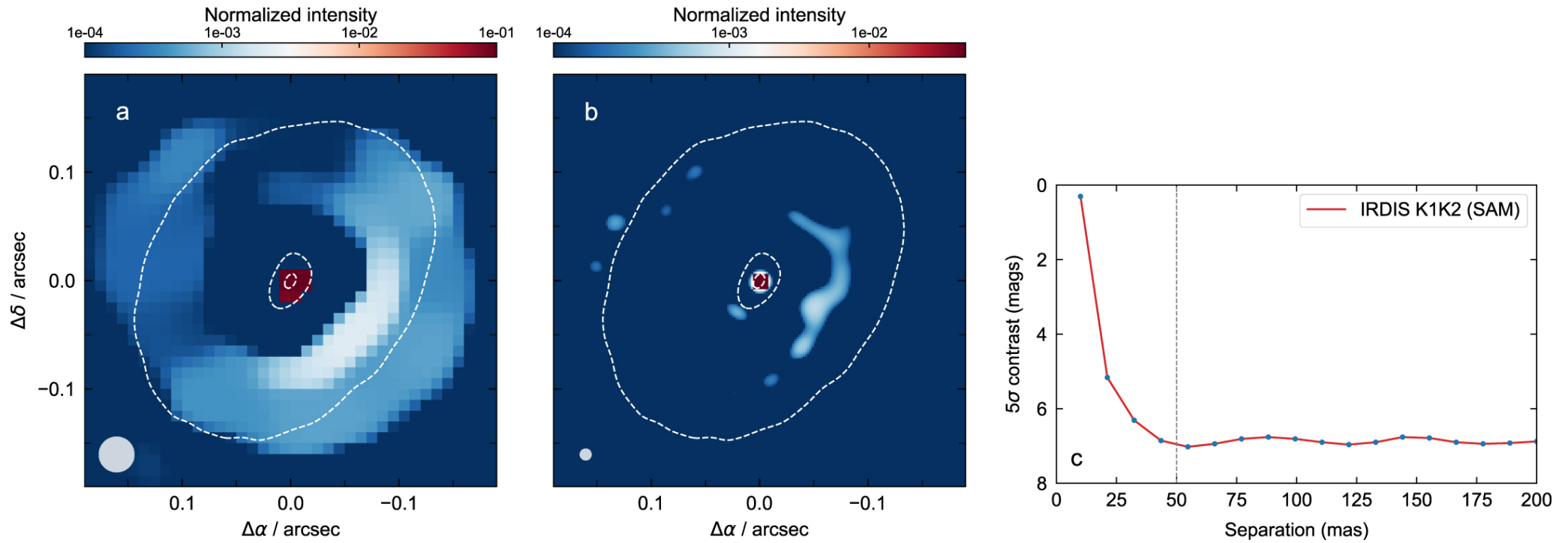
Figure 6. from Long Baseline Observations of the HD 100546 Protoplanetary Disk with ALMA null 2020 APJL 889 L24 doi:10.3847/2041-8213/ab6b2b https://dx.doi.org/10.3847/2041-8213/ab6b2b © 2020. The American Astronomical Society. All rights reserved.
