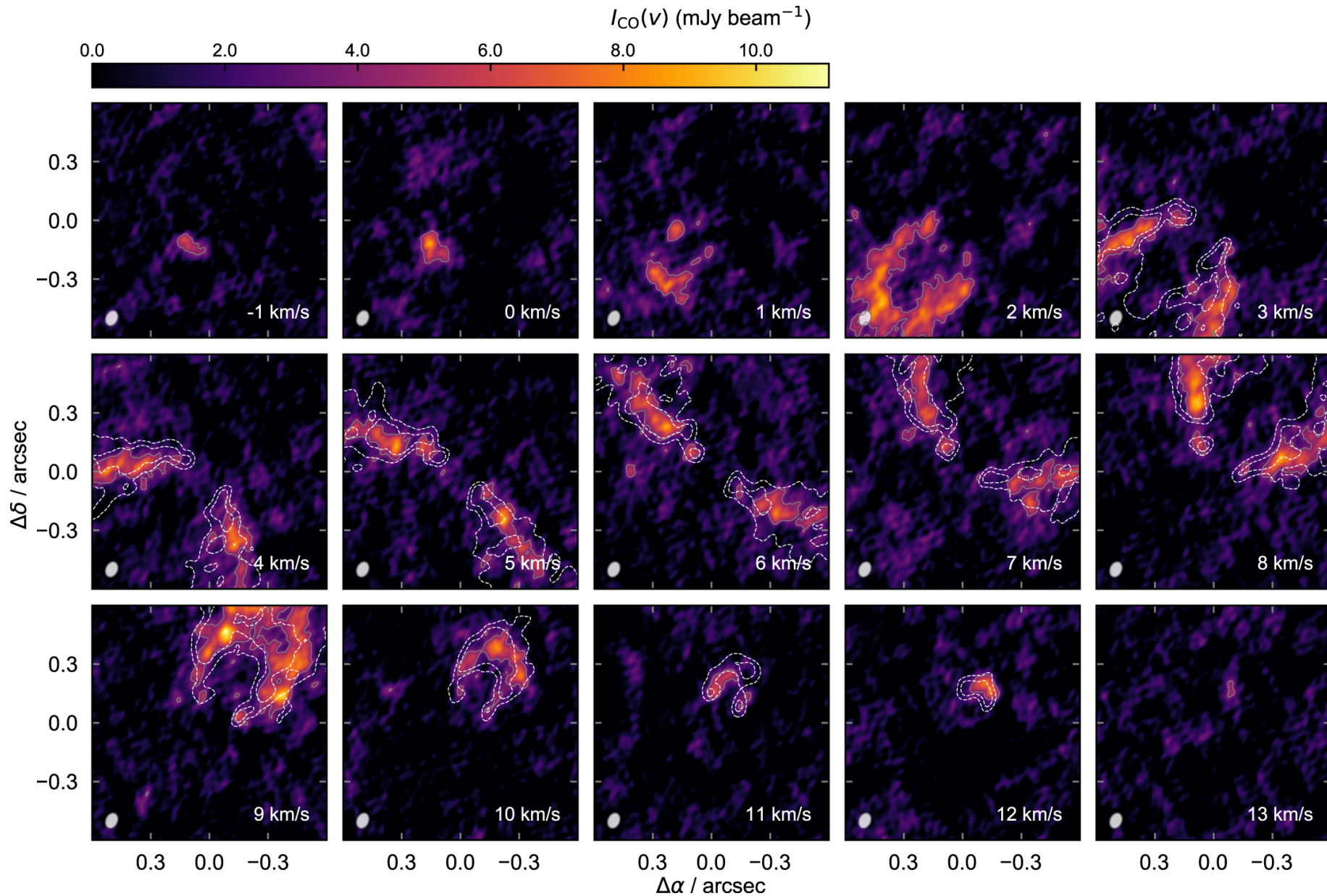
Figure 5. from Long Baseline Observations of the HD 100546 Protoplanetary Disk with ALMA null 2020 APJL 889 L24 doi:10.3847/2041-8213/ab6b2b https://dx.doi.org/10.3847/2041-8213/ab6b2b © 2020. The American Astronomical Society. All rights reserved.
