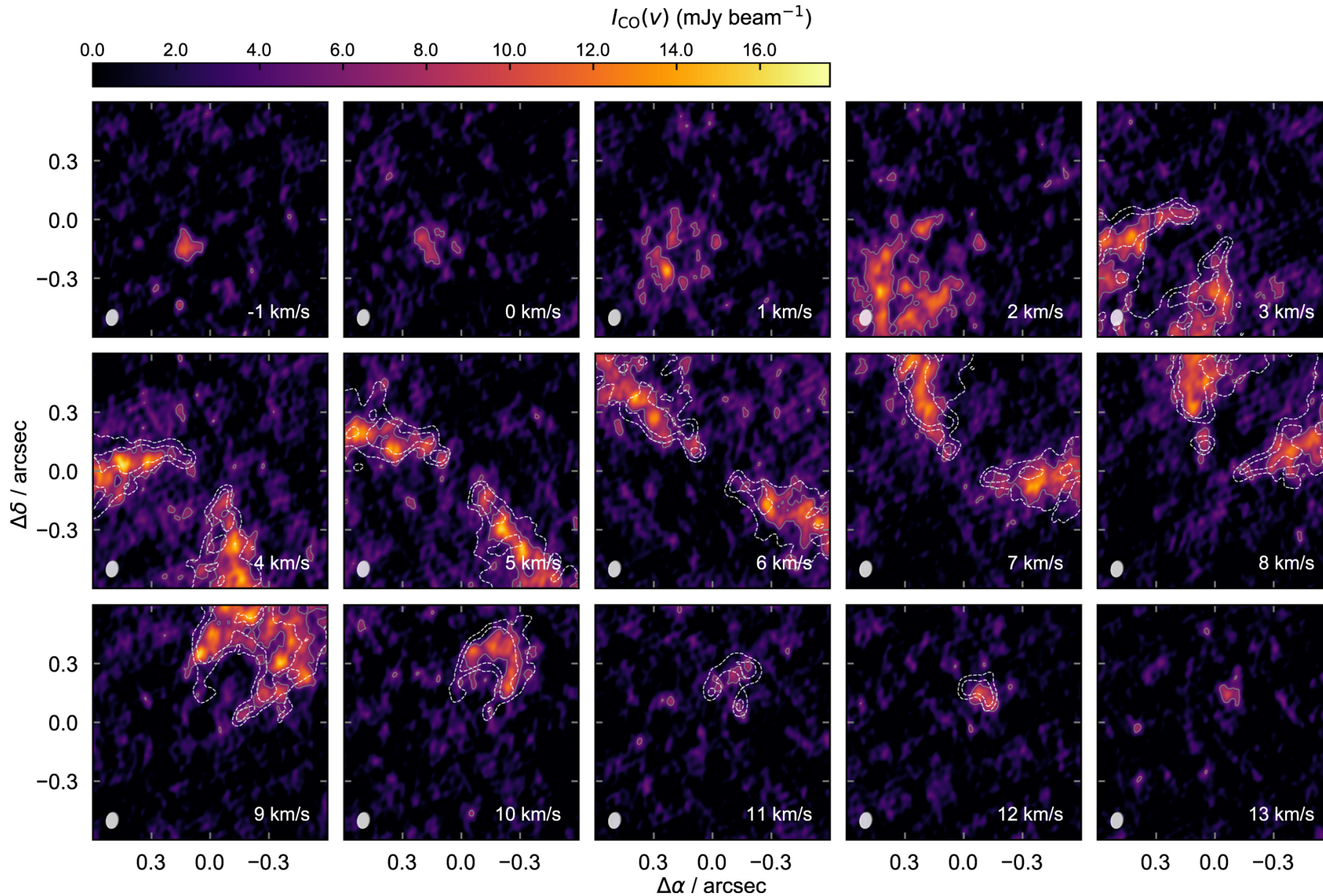
Figure 4. from Long Baseline Observations of the HD 100546 Protoplanetary Disk with ALMA null 2020 APJL 889 L24 doi:10.3847/2041-8213/ab6b2b https://dx.doi.org/10.3847/2041-8213/ab6b2b © 2020. The American Astronomical Society. All rights reserved.
