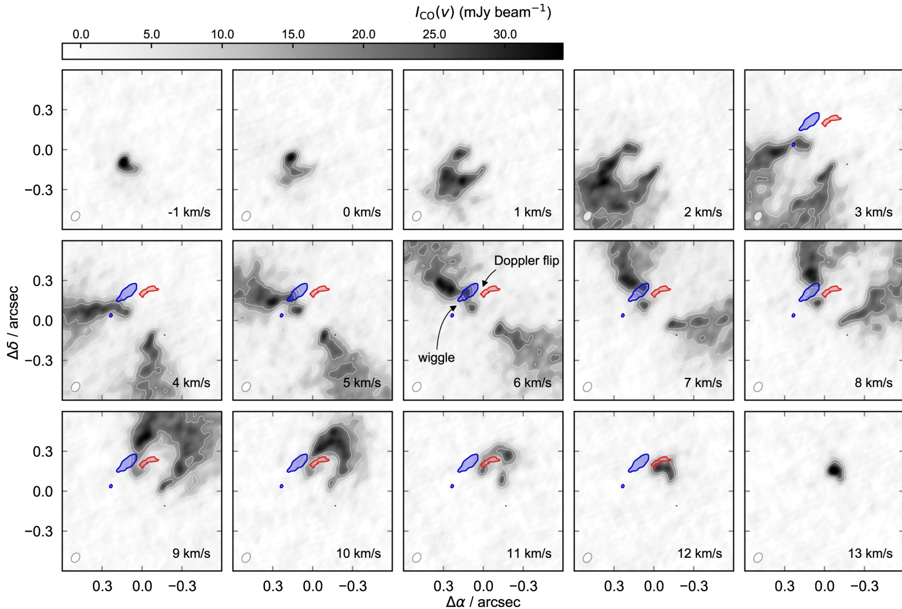
Figure 3. from Long Baseline Observations of the HD 100546 Protoplanetary Disk with ALMA null 2020 APJL 889 L24 doi:10.3847/2041-8213/ab6b2b https://dx.doi.org/10.3847/2041-8213/ab6b2b © 2020. The American Astronomical Society. All rights reserved.
