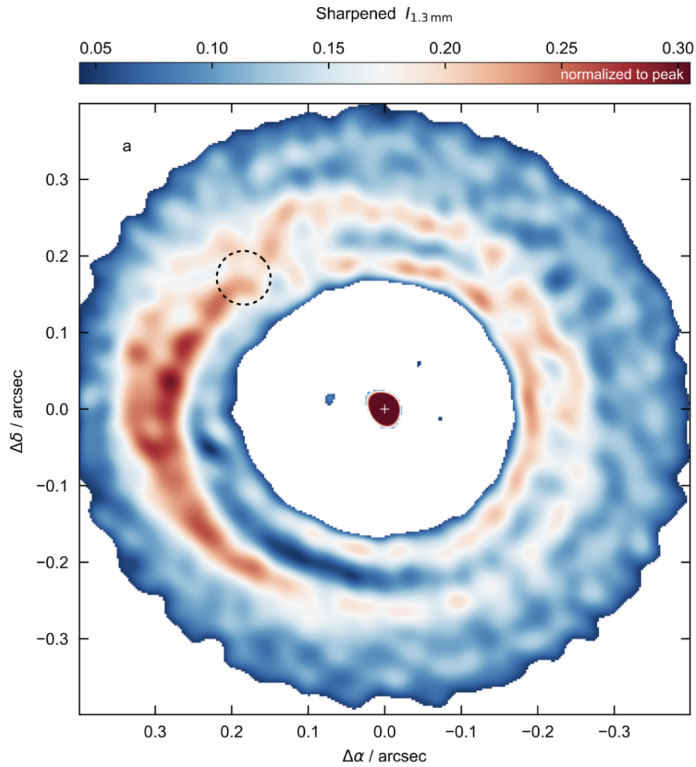
Figure 2. from Long Baseline Observations of the HD 100546 Protoplanetary Disk with ALMA null 2020 APJL 889 L24 doi:10.3847/2041-8213/ab6b2b https://dx.doi.org/10.3847/2041-8213/ab6b2b © 2020. The American Astronomical Society. All rights reserved.
