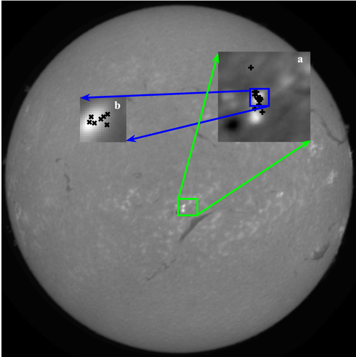
Figure 4. from New Evidence for Spatio-temporal Fragmentation in the Solar Flare Energy Release null 2020 APJL 889 L25 doi:10.3847/2041-8213/ab6a9c https://dx.doi.org/10.3847/2041-8213/ab6a9c © 2020. The American Astronomical Society. All rights reserved.
