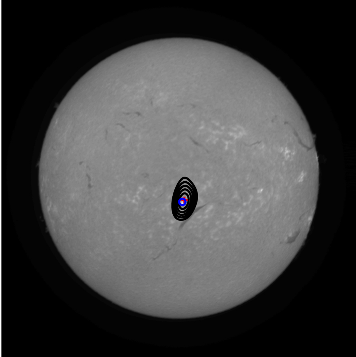
Figure 2. from New Evidence for Spatio-temporal Fragmentation in the Solar Flare Energy Release null 2020 APJL 889 L25 doi:10.3847/2041-8213/ab6a9c https://dx.doi.org/10.3847/2041-8213/ab6a9c © 2020. The American Astronomical Society. All rights reserved.
