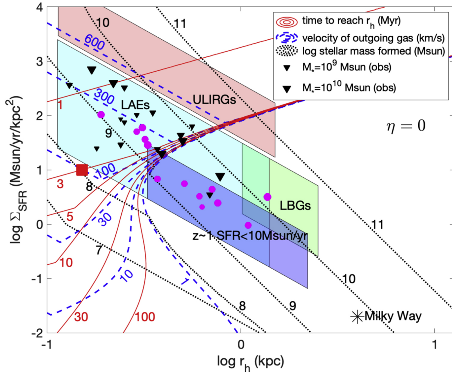
Figure 2. from Physics of Prodigious Lyman Continuum Leakers null 2020 APJL 889 L22 doi:10.3847/2041-8213/ab6560 https://dx.doi.org/10.3847/2041-8213/ab6560 © 2020. The American Astronomical Society. All rights reserved.
