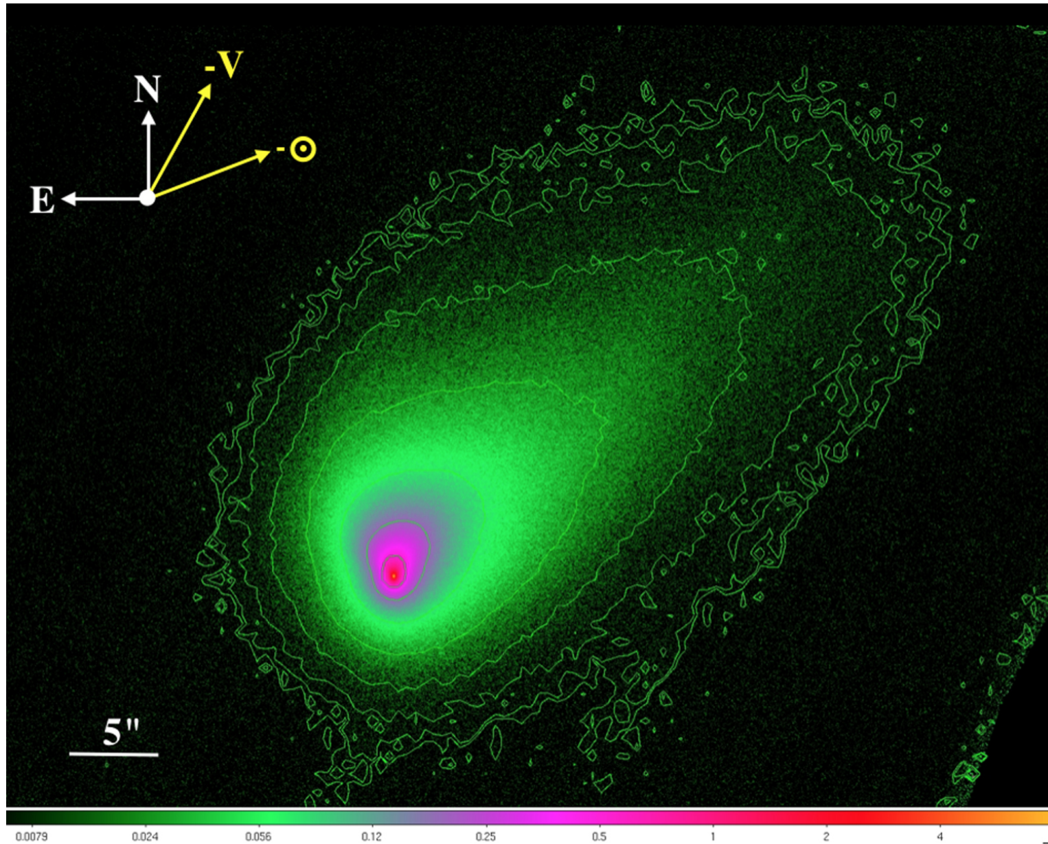
Figure 1. from The Nucleus of Interstellar Comet 2I/Borisov null 2020 APJL 888 L23 doi:10.3847/2041-8213/ab621b https://dx.doi.org/10.3847/2041-8213/ab621b © 2020. The American Astronomical Society. All rights reserved.
