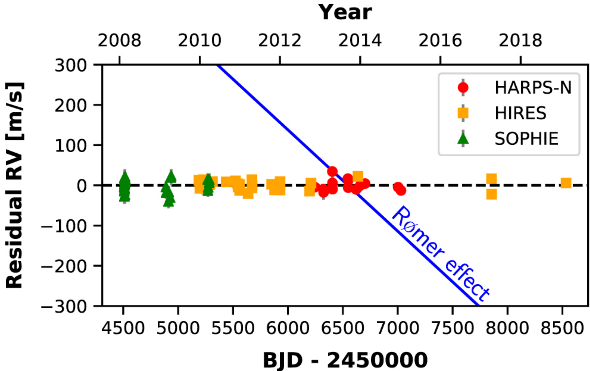
Figure 5. from The Orbit of WASP-12b Is Decaying null 2020 APJL 888 L5 doi:10.3847/2041-8213/ab5c16 https://dx.doi.org/10.3847/2041-8213/ab5c16 © 2019. The American Astronomical Society. All rights reserved.
