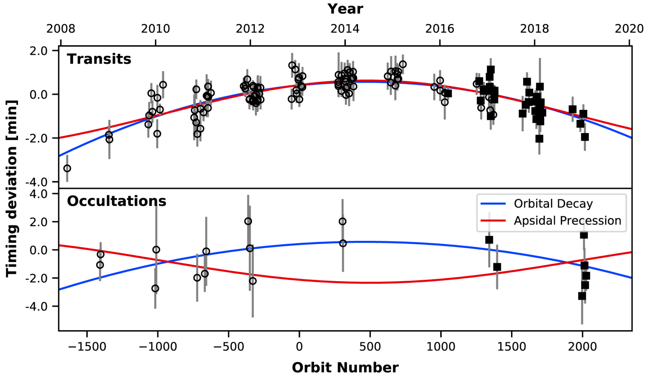
Figure 4. from The Orbit of WASP-12b Is Decaying null 2020 APJL 888 L5 doi:10.3847/2041-8213/ab5c16 https://dx.doi.org/10.3847/2041-8213/ab5c16 © 2019. The American Astronomical Society. All rights reserved.
