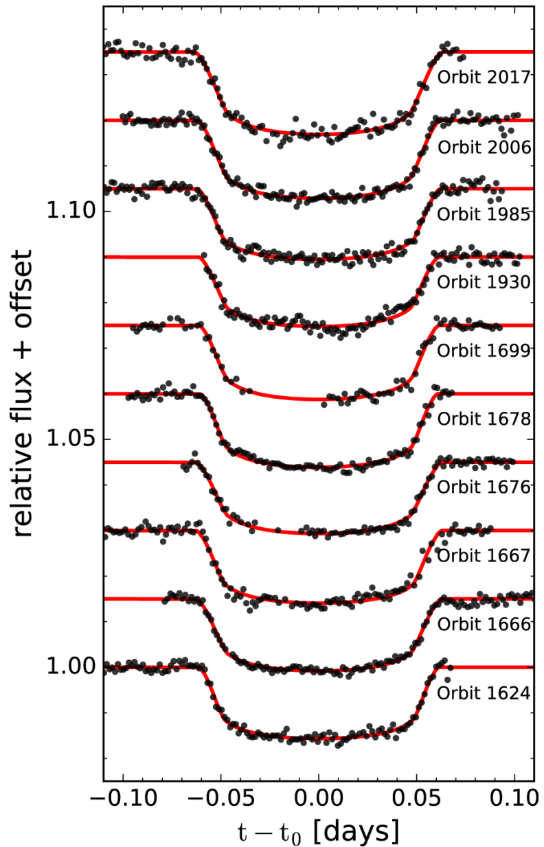
Figure 1. from The Orbit of WASP-12b Is Decaying null 2020 APJL 888 L5 doi:10.3847/2041-8213/ab5c16 https://dx.doi.org/10.3847/2041-8213/ab5c16
