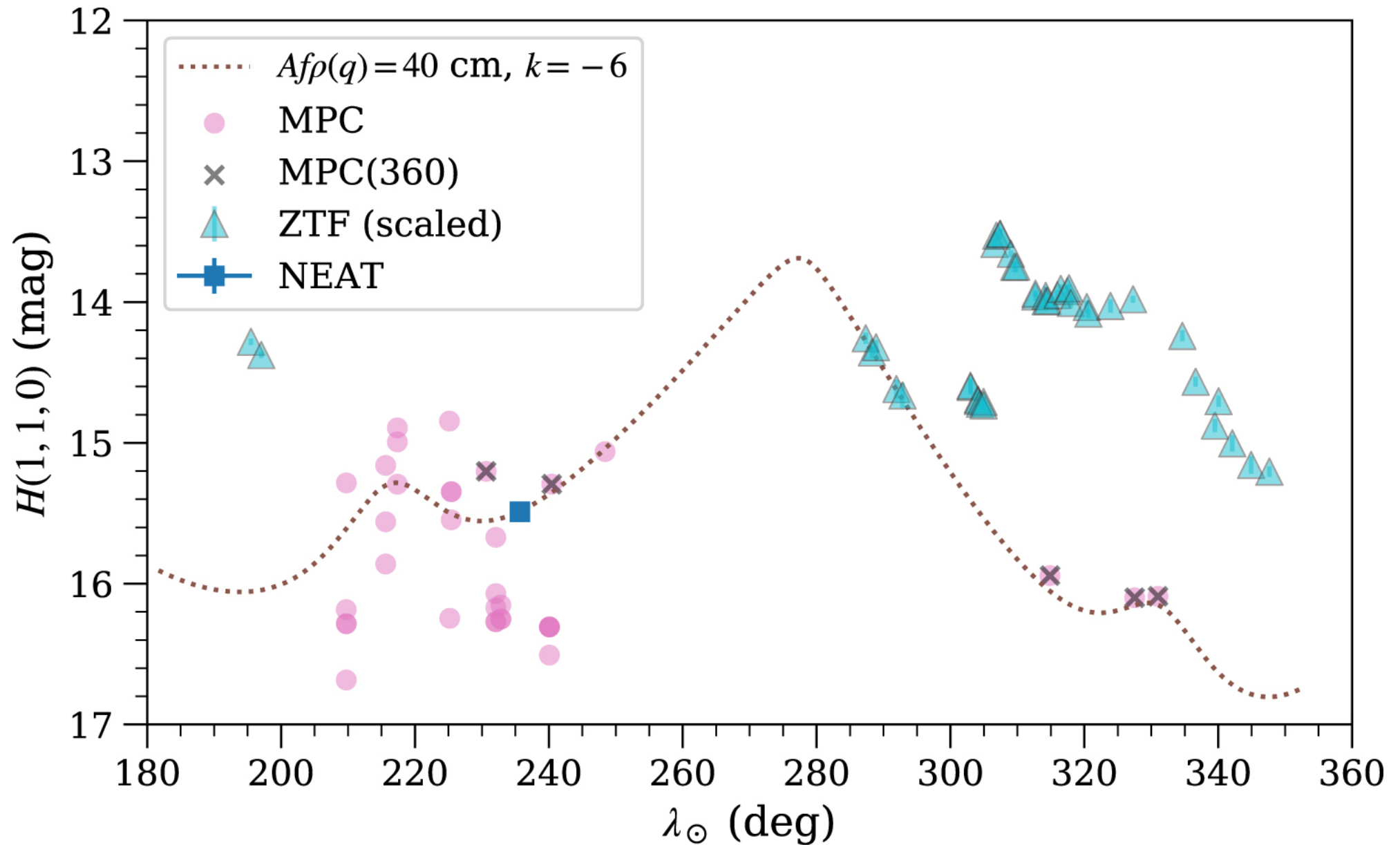
Figure 4. from Comet 240P/NEAT Is Stirring null 2019 APJL 886 L16 doi:10.3847/2041-8213/ab53e0 https://dx.doi.org/10.3847/2041-8213/ab53e0 © 2019. The American Astronomical Society. All rights reserved.
