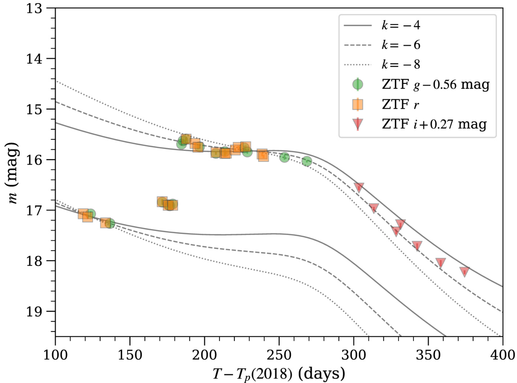
Figure 1. from Comet 240P/NEAT Is Stirring null 2019 APJL 886 L16 doi:10.3847/2041-8213/ab53e0 https://dx.doi.org/10.3847/2041-8213/ab53e0 © 2019. The American Astronomical Society. All rights reserved.
