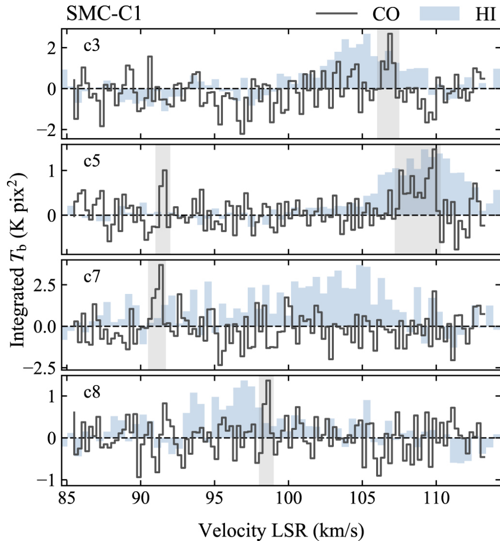
Figure 3. from Molecular Gas in the Outflow of the Small Magellanic Cloud null 2019 APJL 885 L32 doi:10.3847/2041-8213/ab4fe9 https://dx.doi.org/10.3847/2041-8213/ab4fe9 © 2019. The American Astronomical Society. All rights reserved.
