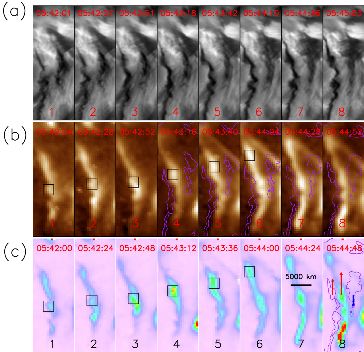
Figure 2. from Multilayered Kelvin–Helmholtz Instability in the Solar Corona null 2019 APJL 884 L51 doi:10.3847/2041-8213/ab4bcd https://dx.doi.org/10.3847/2041-8213/ab4bcd © 2019. The American Astronomical Society. All rights reserved.
