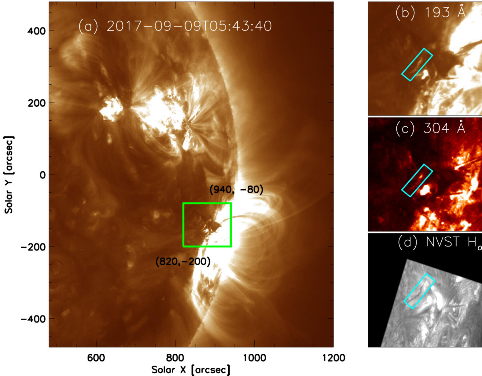
Figure 1. from Multilayered Kelvin–Helmholtz Instability in the Solar Corona null 2019 APJL 884 L51 doi:10.3847/2041-8213/ab4bcd https://dx.doi.org/10.3847/2041-8213/ab4bcd © 2019. The American Astronomical Society. All rights reserved.
