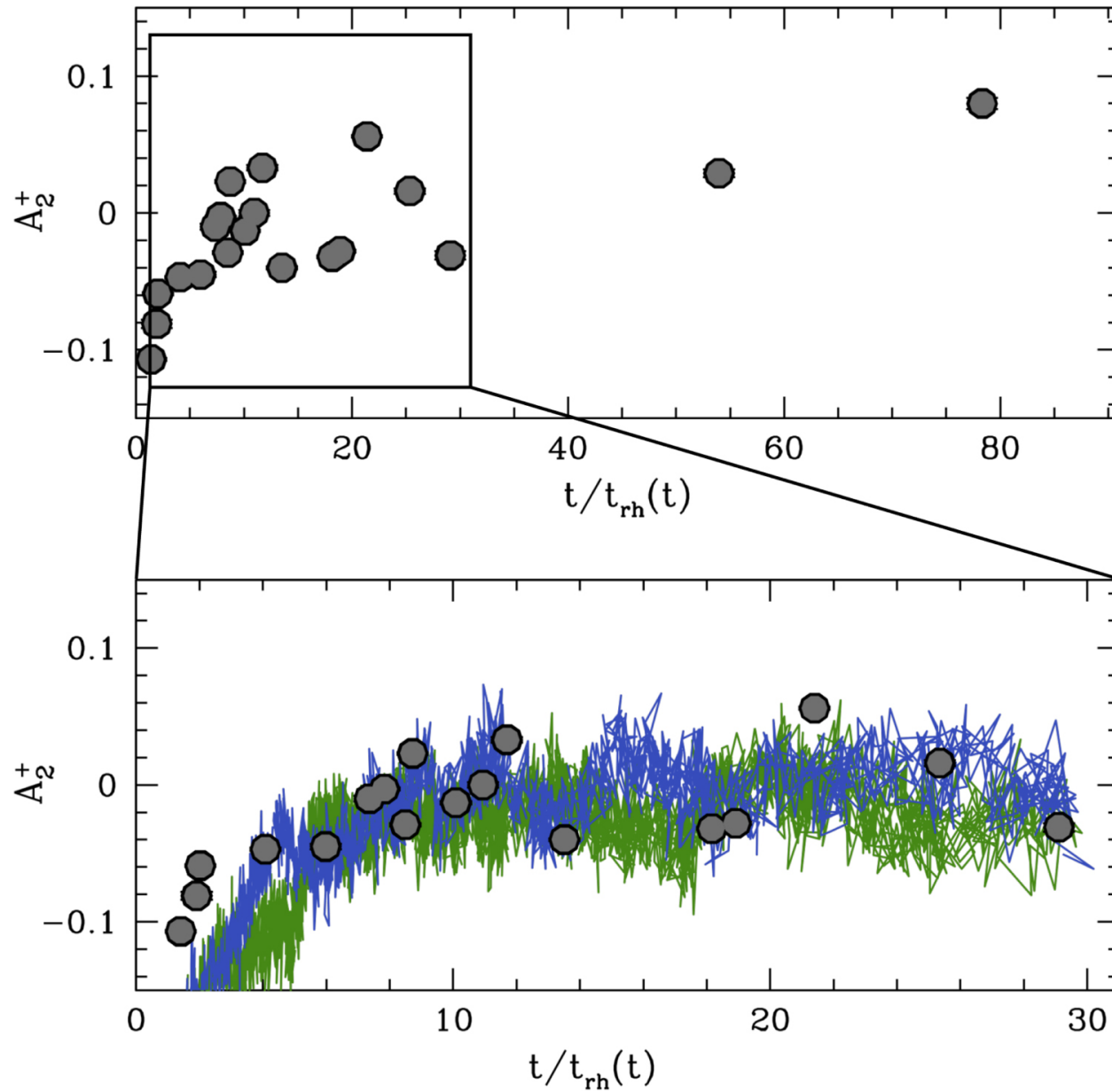
Figure 3. from A Family Picture: Tracing the Dynamical Path of the Structural Properties of Multiple Populations in Globular Clusters null 2019 APJL 884 L24 doi:10.3847/2041-8213/ab45f7 https://dx.doi.org/10.3847/2041-8213/ab45f7 © 2019. The American Astronomical Society. All rights reserved.
