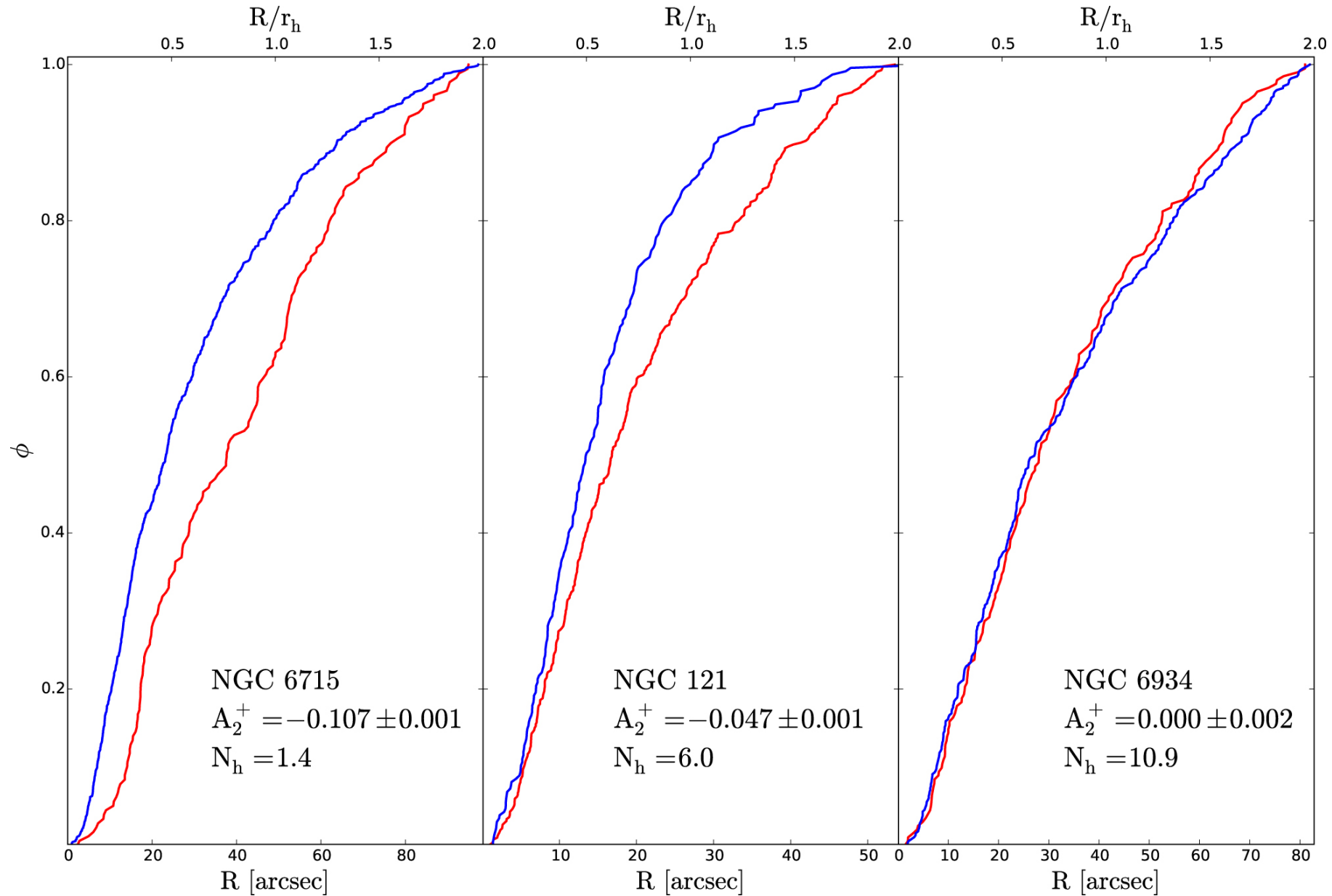
Figure 2. from A Family Picture: Tracing the Dynamical Path of the Structural Properties of Multiple Populations in Globular Clusters null 2019 APJL 884 L24 doi:10.3847/2041-8213/ab45f7 https://dx.doi.org/10.3847/2041-8213/ab45f7 © 2019. The American Astronomical Society. All rights reserved.
