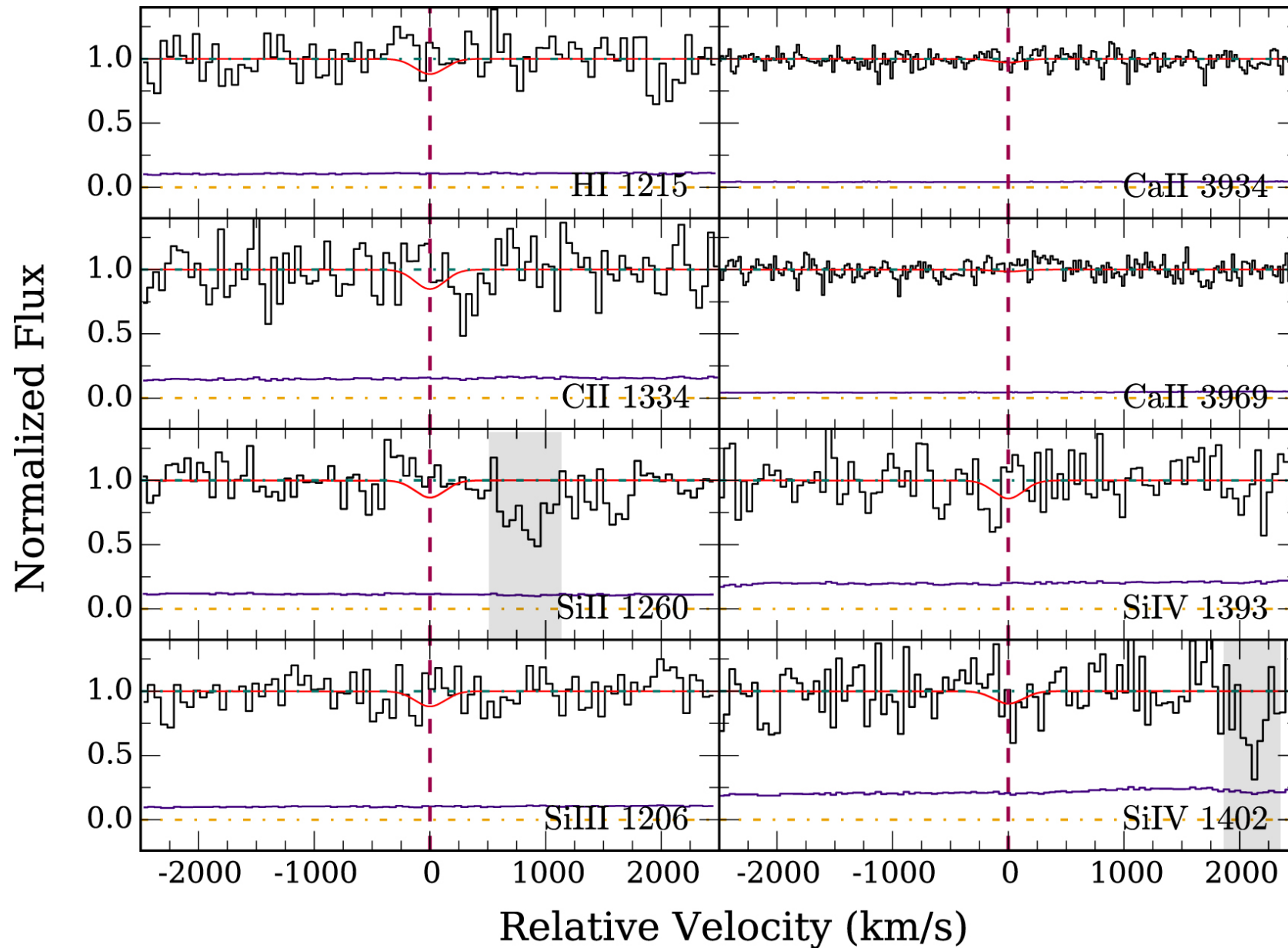
Figure 3. from COS Observations of the Cosmic Web: A Search for the Cooler Components of a Hot, X-Ray Identified Filament null 2019 APJL 884 L20 doi:10.3847/2041-8213/ab45f5 https://dx.doi.org/10.3847/2041-8213/ab45f5 © 2019. The American Astronomical Society. All rights reserved.
