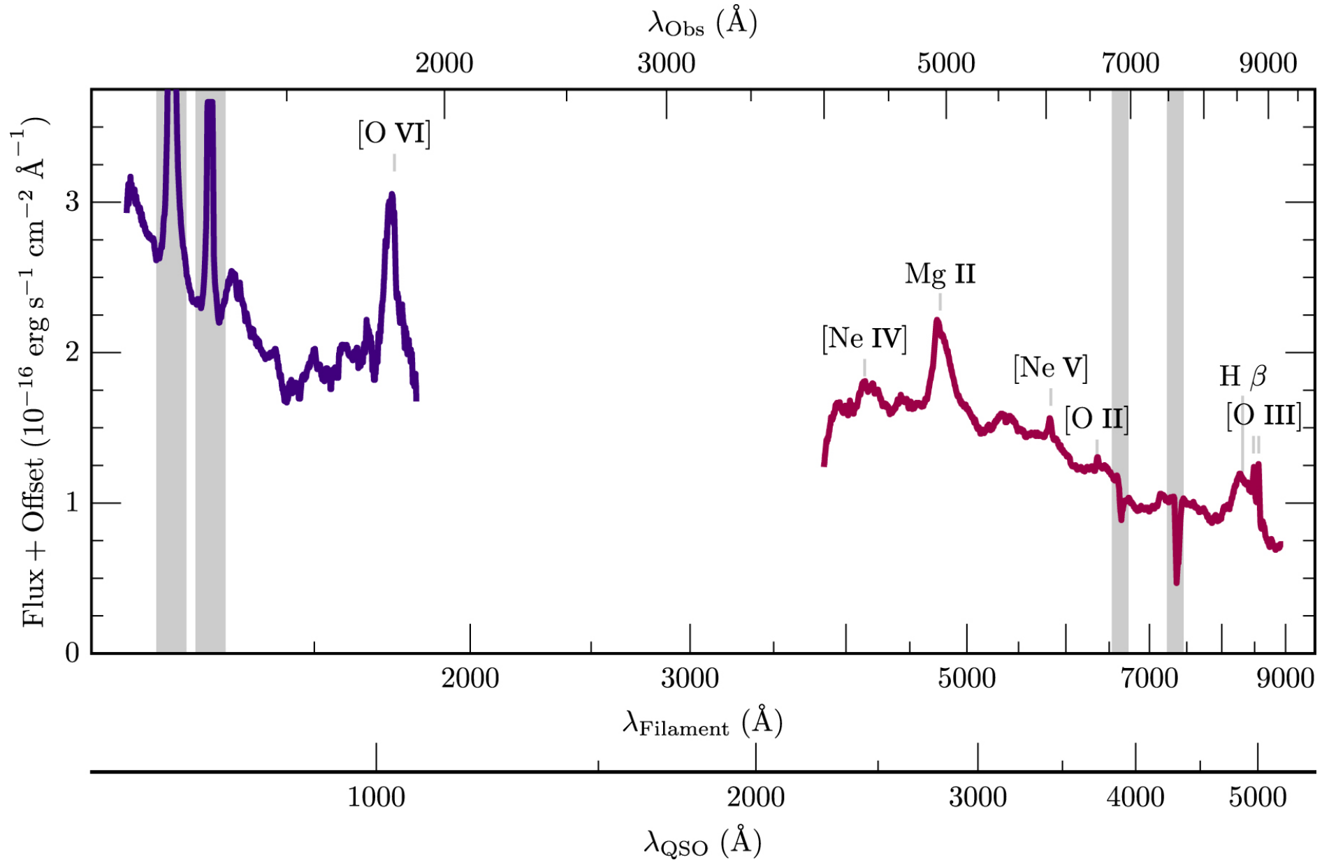
Figure 2. from COS Observations of the Cosmic Web: A Search for the Cooler Components of a Hot, X-Ray Identified Filament null 2019 APJL 884 L20 doi:10.3847/2041-8213/ab45f5 https://dx.doi.org/10.3847/2041-8213/ab45f5 © 2019. The American Astronomical Society. All rights reserved.
