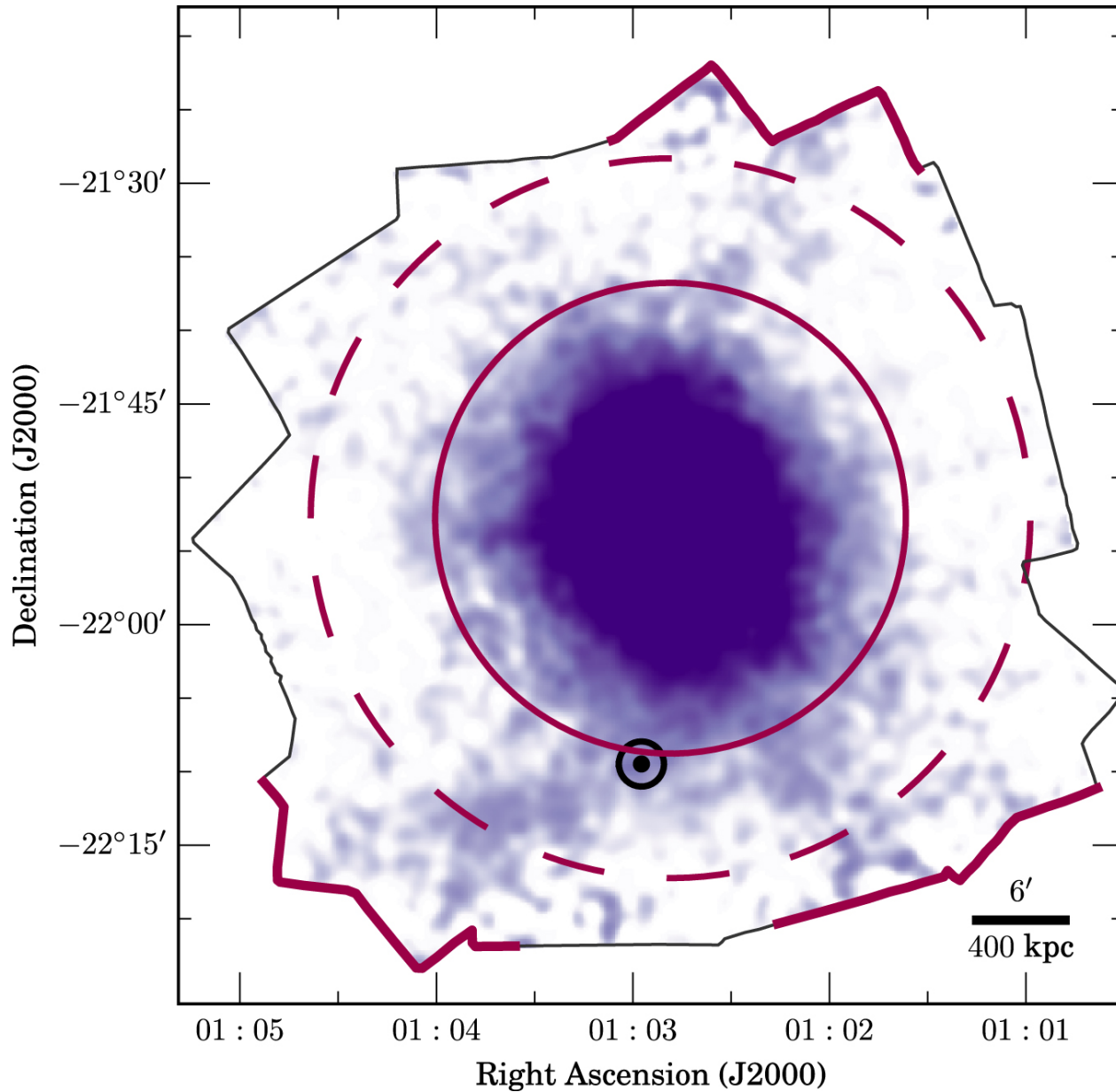
Figure 1. from COS Observations of the Cosmic Web: A Search for the Cooler Components of a Hot, X-Ray Identified Filament null 2019 APJL 884 L20 doi:10.3847/2041-8213/ab45f5 https://dx.doi.org/10.3847/2041-8213/ab45f5 © 2019. The American Astronomical Society. All rights reserved.
