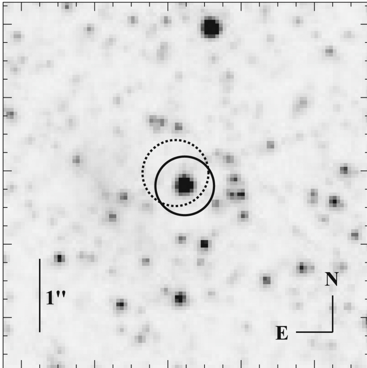
Figure 6. from Discovery of a Red Supergiant Donor Star in SN2010da/NGC 300 ULX-1 null 2019 APJL 883 L34 doi:10.3847/2041-8213/ab4139 https://dx.doi.org/10.3847/2041-8213/ab4139 © 2019. The American Astronomical Society. All rights reserved.
