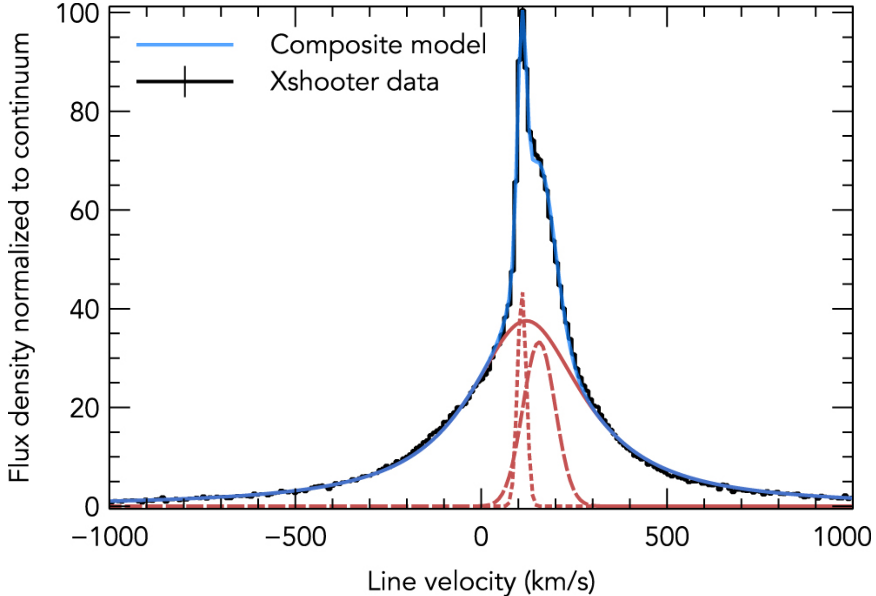
Figure 4. from Discovery of a Red Supergiant Donor Star in SN2010da/NGC 300 ULX-1 null 2019 APJL 883 L34 doi:10.3847/2041-8213/ab4139 https://dx.doi.org/10.3847/2041-8213/ab4139 © 2019. The American Astronomical Society. All rights reserved.
