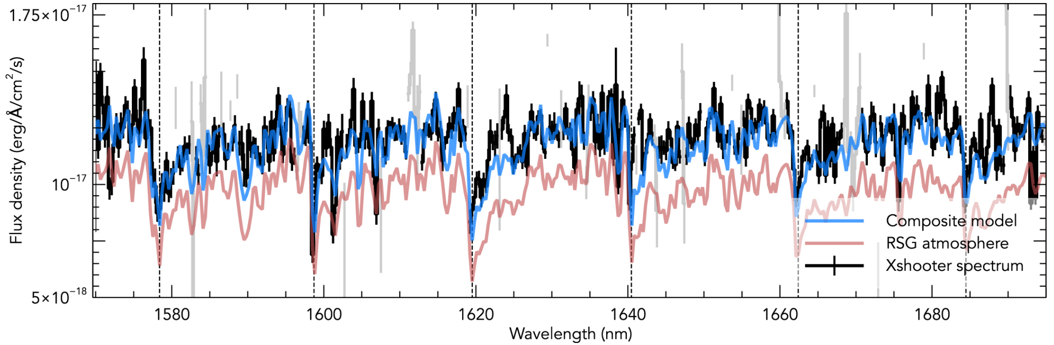
Figure 3. from Discovery of a Red Supergiant Donor Star in SN2010da/NGC 300 ULX-1 null 2019 APJL 883 L34 doi:10.3847/2041-8213/ab4139 https://dx.doi.org/10.3847/2041-8213/ab4139 © 2019. The American Astronomical Society. All rights reserved.
