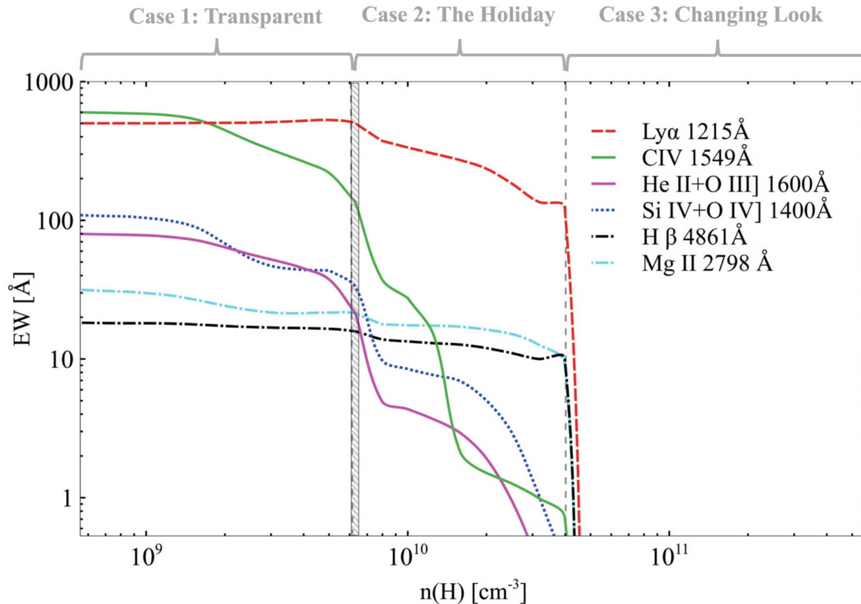
Figure 4. from A Wind-based Unification Model for NGC 5548: Spectral Holidays, Nondisk Emission, and Implications for Changing-look Quasars null 2019 APJL 882 L30 doi:10.3847/2041-8213/ab3d41 https://dx.doi.org/10.3847/2041-8213/ab3d41 © 2019. The American Astronomical Society. All rights reserved.
