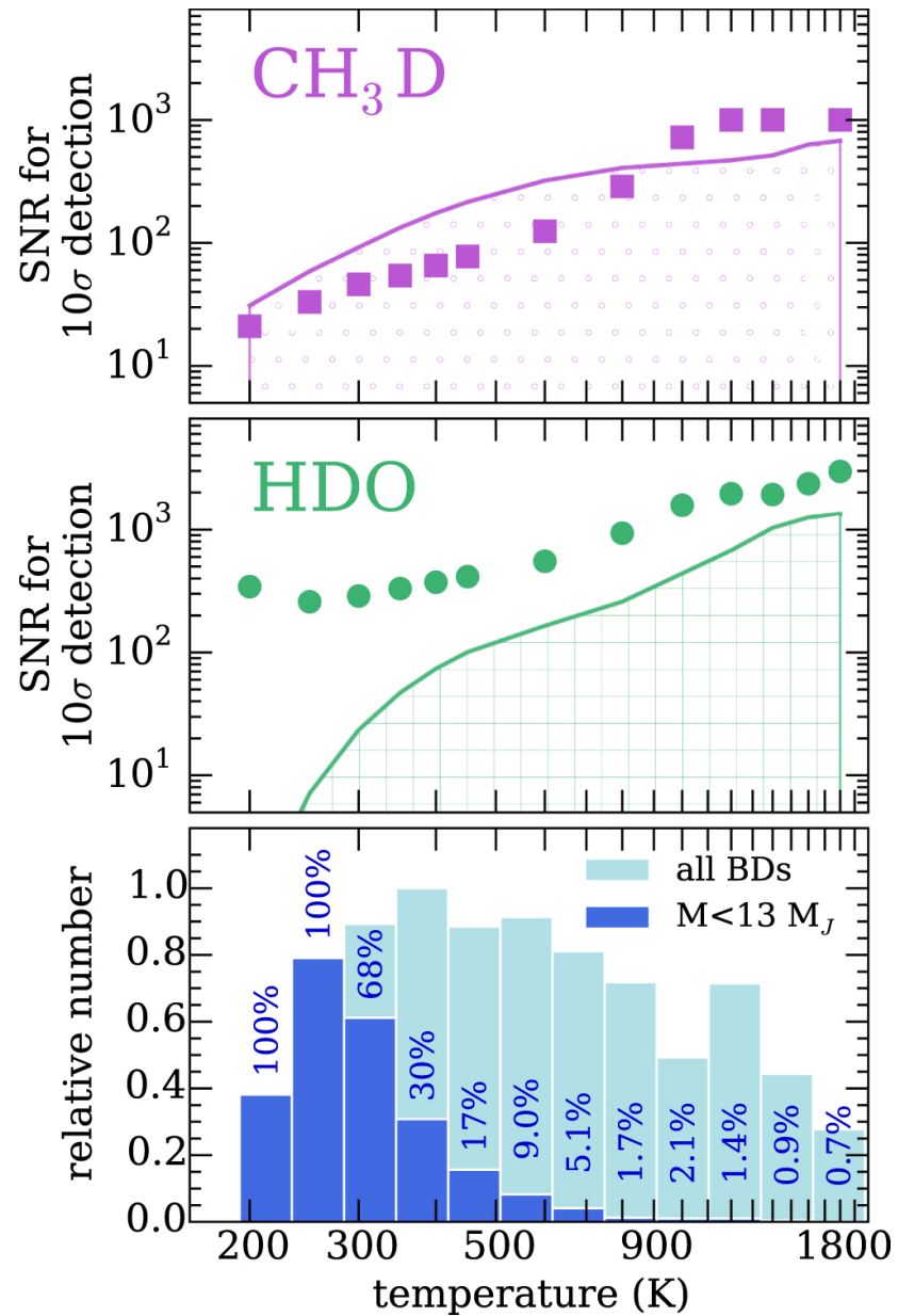
Figure 4. from Measuring the D/H Ratios of Exoplanets and Brown Dwarfs null 2019 APJL 882 L29 doi:10.3847/2041-8213/ab3c65 https://dx.doi.org/10.3847/2041-8213/ab3c65 © 2019. The American Astronomical Society. All rights reserved.
