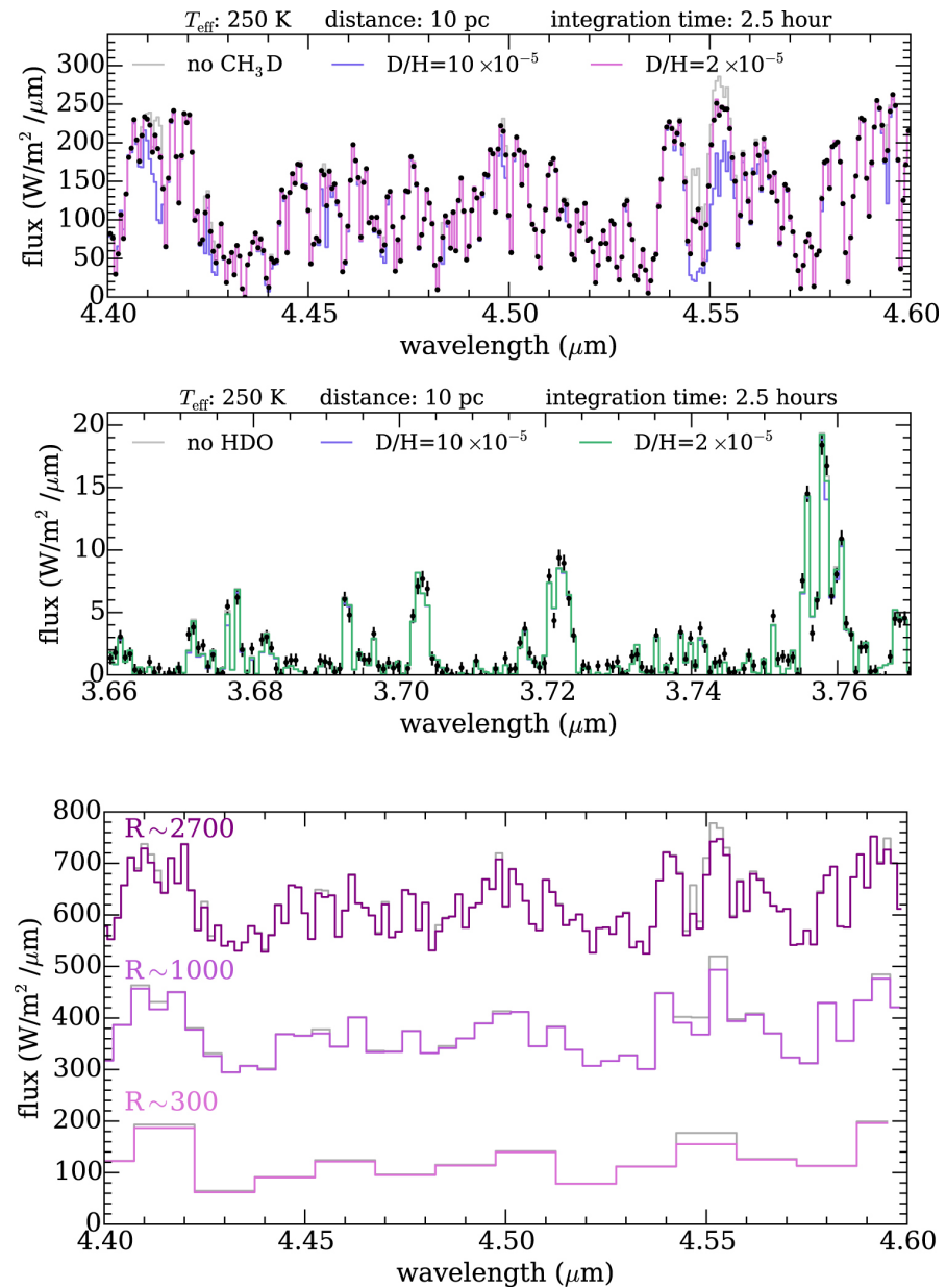
Figure 3. from Measuring the D/H Ratios of Exoplanets and Brown Dwarfs null 2019 APJL 882 L29 doi:10.3847/2041-8213/ab3c65 https://dx.doi.org/10.3847/2041-8213/ab3c65 © 2019. The American Astronomical Society. All rights reserved.
