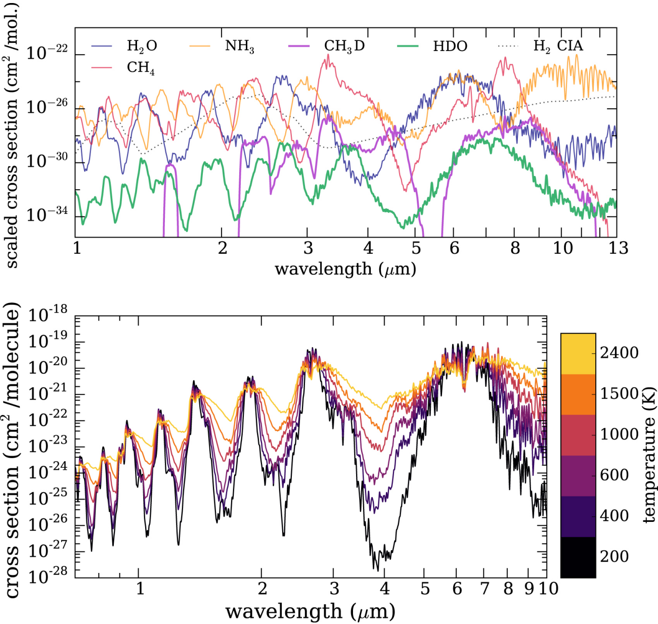
Figure 2. from Measuring the D/H Ratios of Exoplanets and Brown Dwarfs null 2019 APJL 882 L29 doi:10.3847/2041-8213/ab3c65 https://dx.doi.org/10.3847/2041-8213/ab3c65 © 2019. The American Astronomical Society. All rights reserved.
