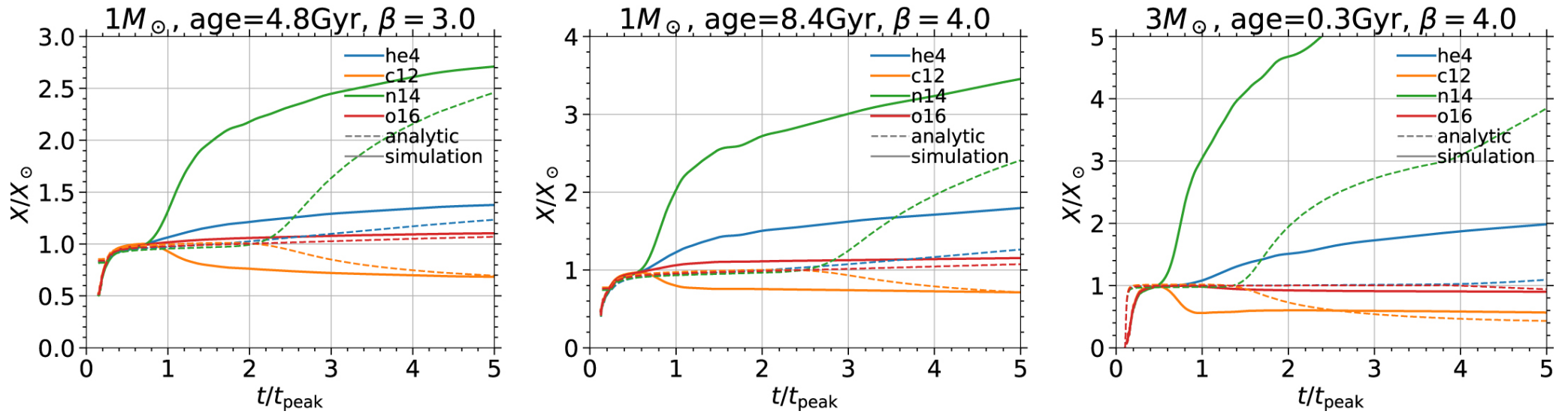
Figure 5. from The Tidal Disruption of Sun-like Stars by Massive Black Holes null 2019 APJL 882 L25 doi:10.3847/2041-8213/ab379a https://dx.doi.org/10.3847/2041-8213/ab379a © 2019. The American Astronomical Society. All rights reserved.
