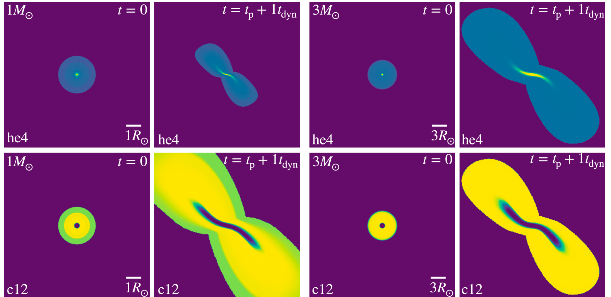
Figure 4. from The Tidal Disruption of Sun-like Stars by Massive Black Holes null 2019 APJL 882 L25 doi:10.3847/2041-8213/ab379a https://dx.doi.org/10.3847/2041-8213/ab379a © 2019. The American Astronomical Society. All rights reserved.
