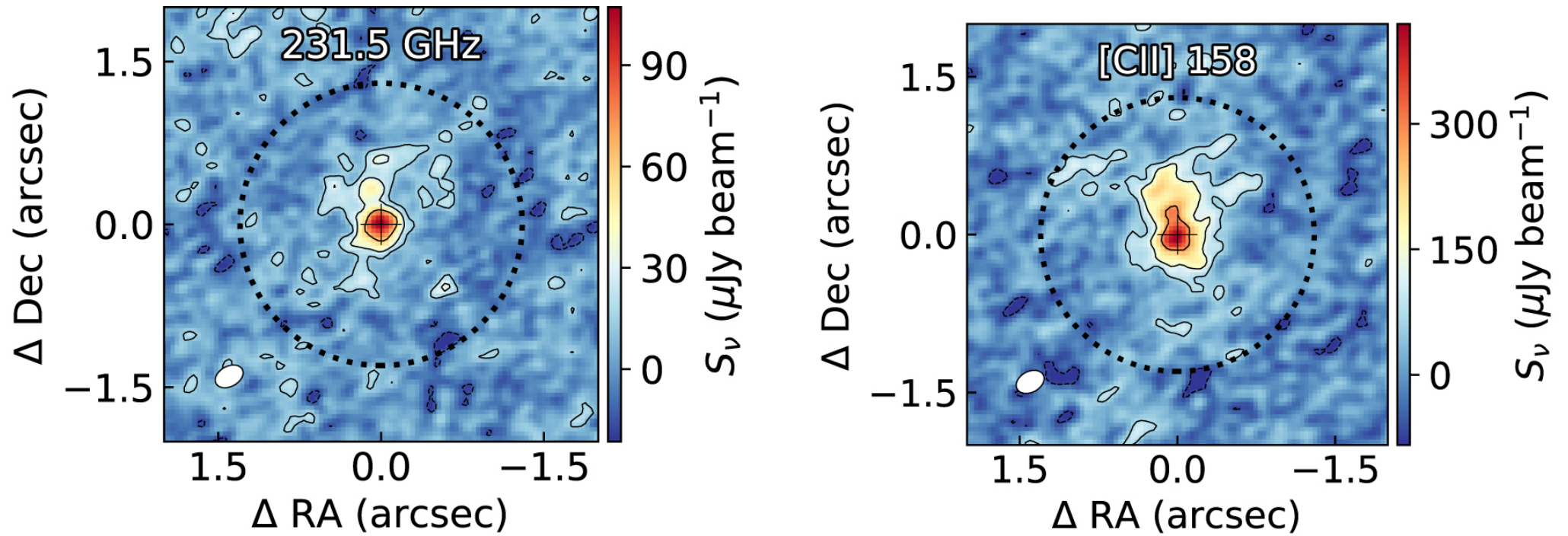
Figure 2. from The z = 7.54 Quasar ULAS J1342+0928 Is Hosted by a Galaxy Merger null 2019 APJL 881 L23 doi:10.3847/2041-8213/ab3659 https://dx.doi.org/10.3847/2041-8213/ab3659 © 2019. The American Astronomical Society. All rights reserved.
