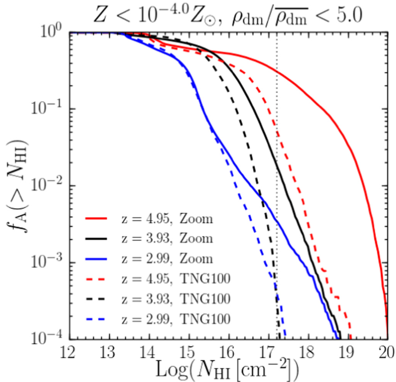
Figure 5. from Shattering of Cosmic Sheets due to Thermal Instabilities: A Formation Channel for Metal-free Lyman Limit Systems null 2019 APJL 881 L20 doi:10.3847/2041-8213/ab30cb https://dx.doi.org/10.3847/2041-8213/ab30cb © 2019. The American Astronomical Society. All rights reserved.
