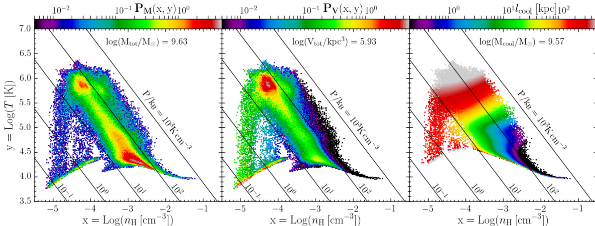
Figure 3. from Shattering of Cosmic Sheets due to Thermal Instabilities: A Formation Channel for Metal-free Lyman Limit Systems null 2019 APJL 881 L20 doi:10.3847/2041-8213/ab30cb https://dx.doi.org/10.3847/2041-8213/ab30cb © 2019. The American Astronomical Society. All rights reserved.
