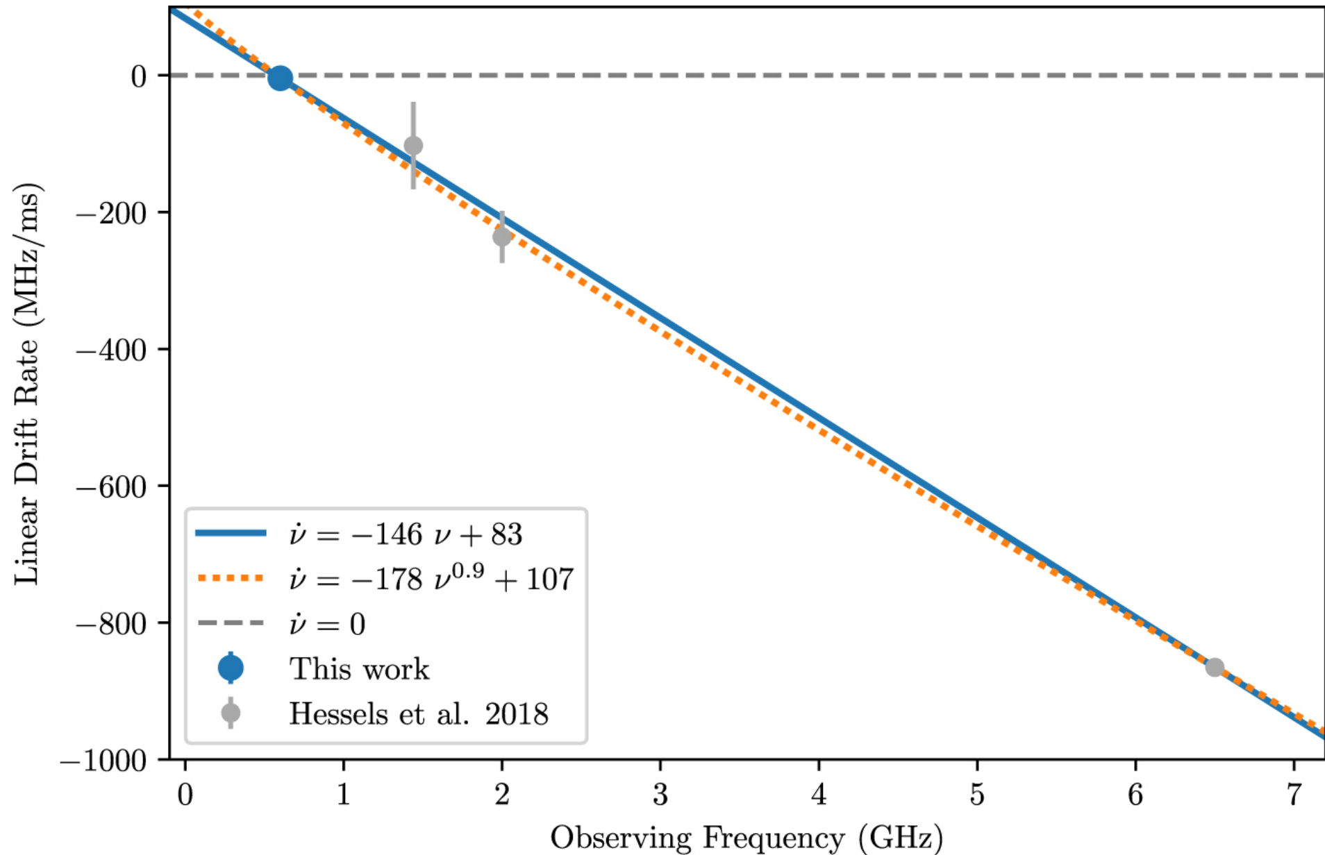
Figure 6. from CHIME/FRB Detection of the Original Repeating Fast Radio Burst Source FRB 121102 null 2019 APJL 882 L18 doi:10.3847/2041-8213/ab2c00 https://dx.doi.org/10.3847/2041-8213/ab2c00 © 2019. The American Astronomical Society. All rights reserved.
