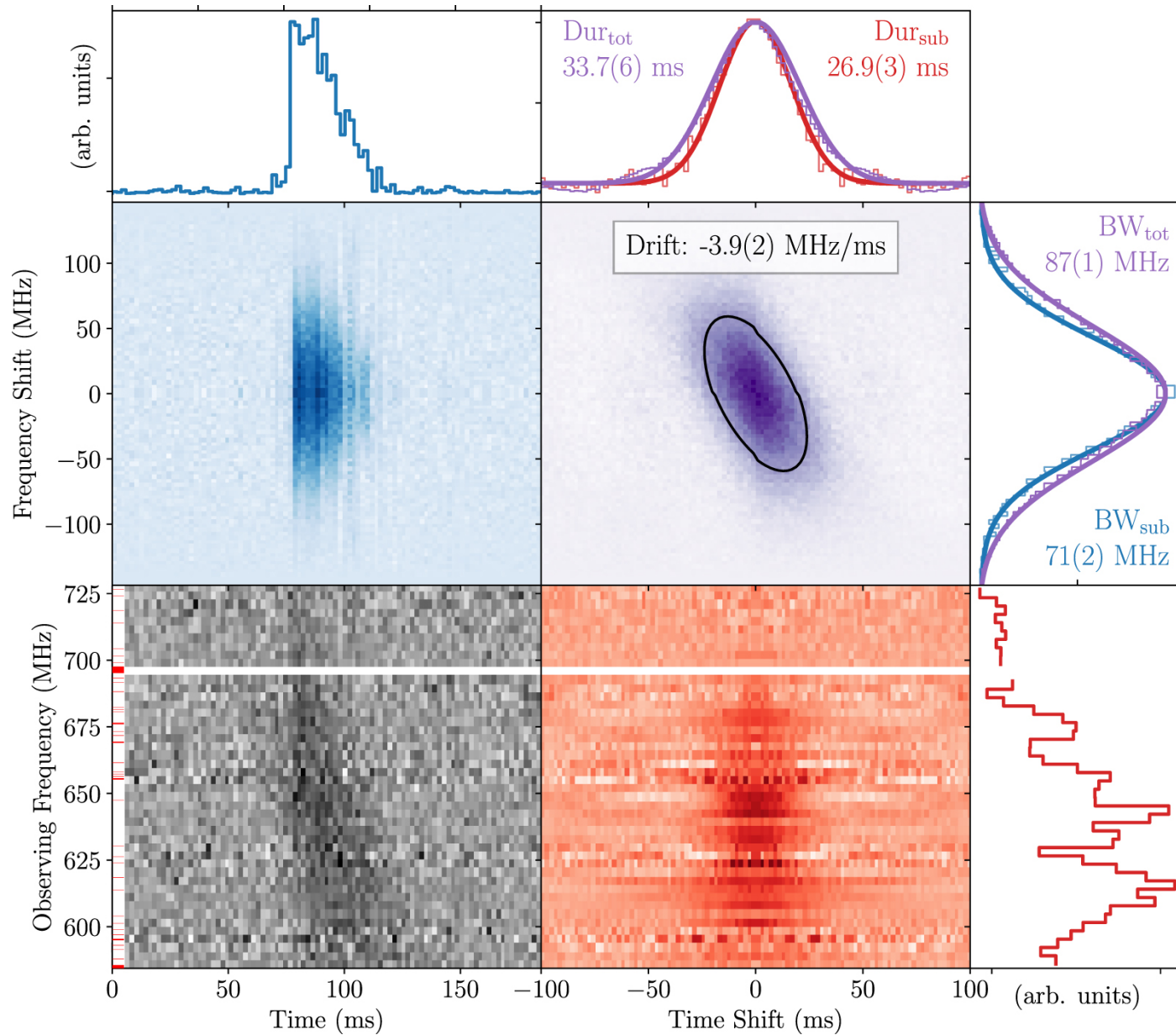
Figure 5. from CHIME/FRB Detection of the Original Repeating Fast Radio Burst Source FRB 121102 null 2019 APJL 882 L18 doi:10.3847/2041-8213/ab2c00 https://dx.doi.org/10.3847/2041-8213/ab2c00 © 2019. The American Astronomical Society. All rights reserved.
