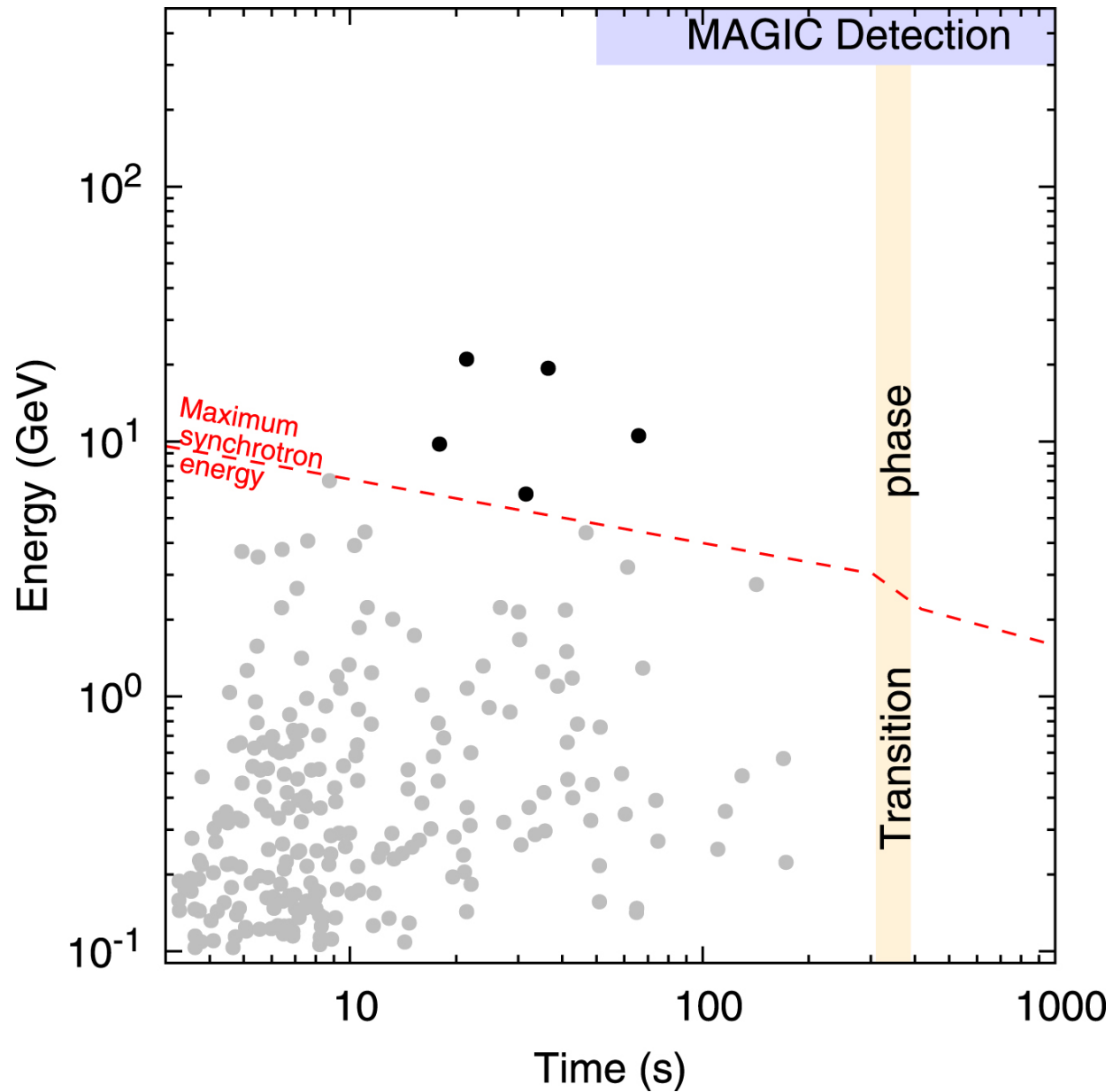
Figure 4. from Analysis and Modeling of the Multi-wavelength Observations of the Luminous GRB 190114C null 2019 APJL 879 L26 doi:10.3847/2041-8213/ab2ae4 https://dx.doi.org/10.3847/2041-8213/ab2ae4 © 2019. The American Astronomical Society. All rights reserved.
