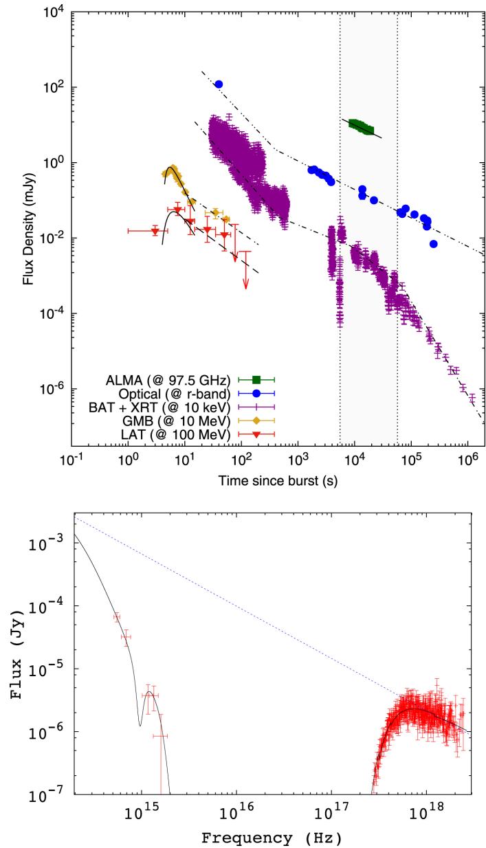
Figure 3. from Analysis and Modeling of the Multi-wavelength Observations of the Luminous GRB 190114C null 2019 APJL 879 L26 doi:10.3847/2041-8213/ab2ae4 https://dx.doi.org/10.3847/2041-8213/ab2ae4 © 2019. The American Astronomical Society. All rights reserved.
