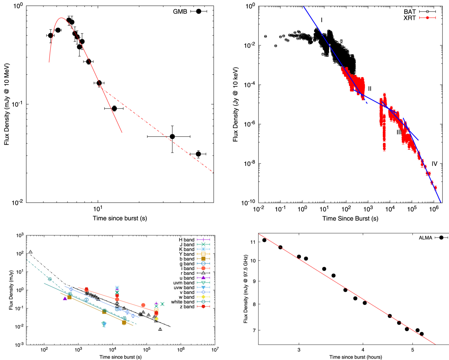
Figure 2. from Analysis and Modeling of the Multi-wavelength Observations of the Luminous GRB 190114C null 2019 APJL 879 L26 doi:10.3847/2041-8213/ab2ae4 https://dx.doi.org/10.3847/2041-8213/ab2ae4 © 2019. The American Astronomical Society. All rights reserved.
