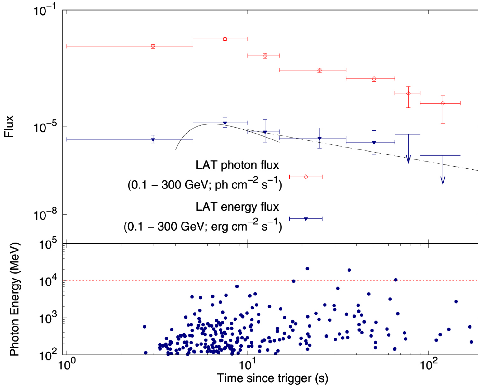
Figure 1. from Analysis and Modeling of the Multi-wavelength Observations of the Luminous GRB 190114C null 2019 APJL 879 L26 doi:10.3847/2041-8213/ab2ae4 https://dx.doi.org/10.3847/2041-8213/ab2ae4 © 2019. The American Astronomical Society. All rights reserved.
