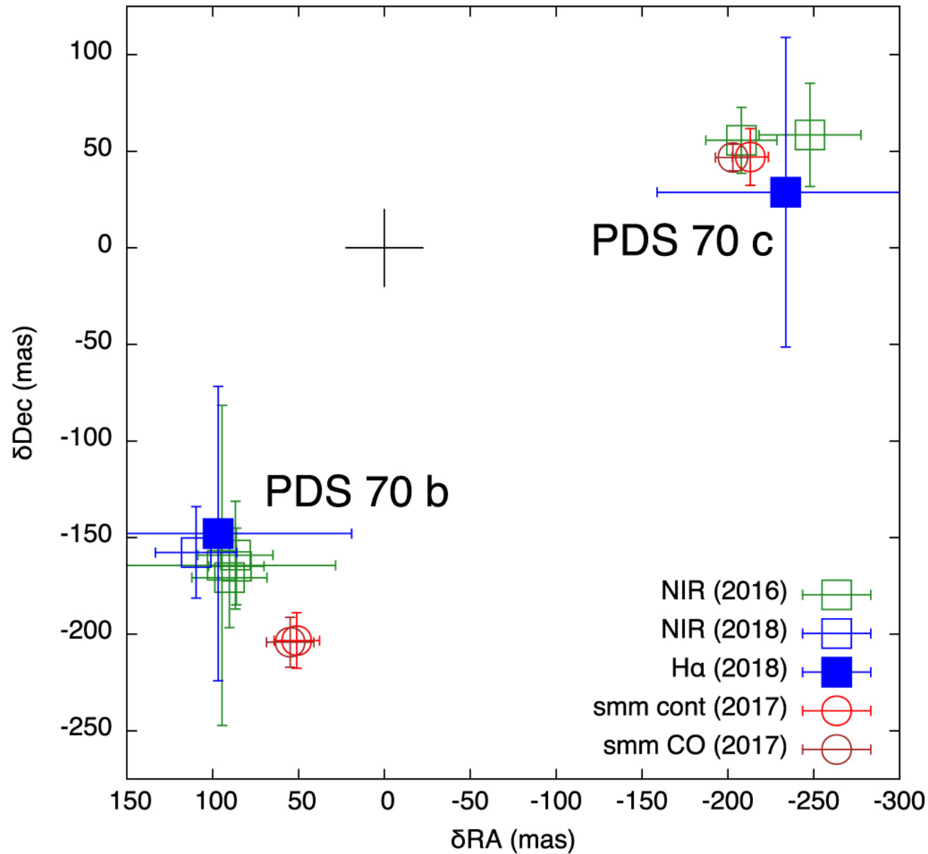
Figure 2. from Detection of Continuum Submillimeter Emission Associated with Candidate Protoplanets null 2019 APJL 879 L25 doi:10.3847/2041-8213/ab2a12 https://dx.doi.org/10.3847/2041-8213/ab2a12 © 2019. The American Astronomical Society. All rights reserved.
