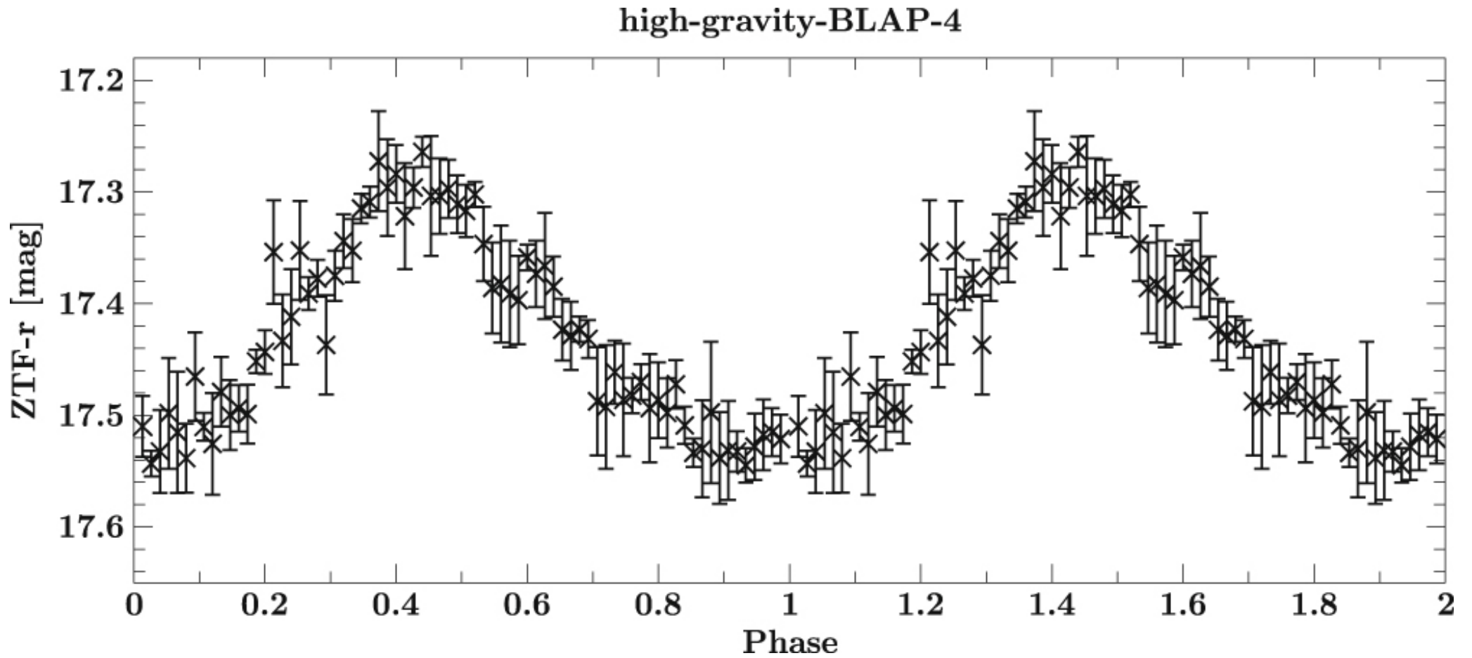
Figure 2. from A New Class of Large-amplitude Radial-mode Hot Subdwarf Pulsators null 2019 APJL 878 L35 doi:10.3847/2041-8213/ab263c https://dx.doi.org/10.3847/2041-8213/ab263c © 2019. The American Astronomical Society. All rights reserved.
