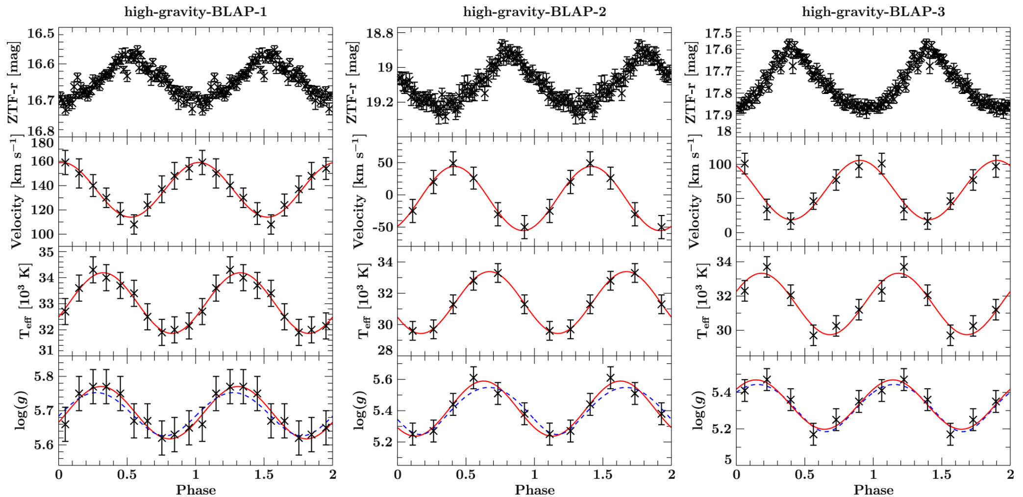
Figure 1. from A New Class of Large-amplitude Radial-mode Hot Subdwarf Pulsators null 2019 APJL 878 L35 doi:10.3847/2041-8213/ab263c https://dx.doi.org/10.3847/2041-8213/ab263c © 2019. The American Astronomical Society. All rights reserved.
